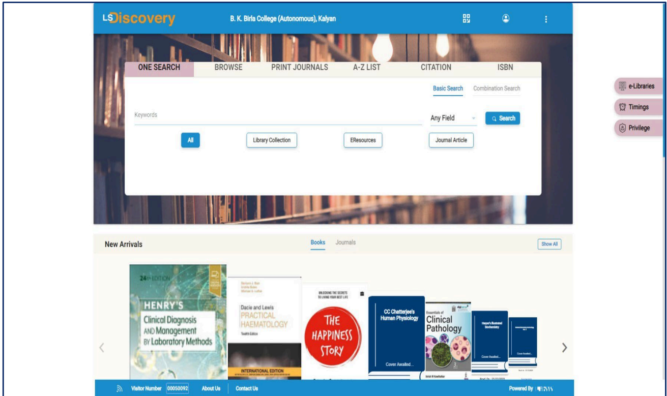
Figure 5 – LSDiscovery
